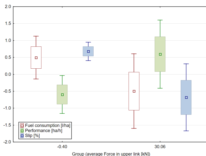
12: The box graph for the tractor in the aggregation with the cultivator, point: average value, box: average \pm standard deviation, whisker: average \pm 1.96 \times standard deviation, standardized data
