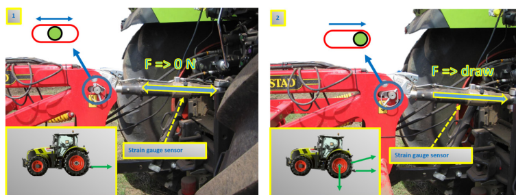
2: Tractor Claas with the tensometer in the upper link of three-point hitch
