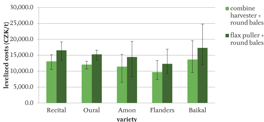
5: Levelized costs for production of linseed selected varieties (related to the mass of seed dry matter)
