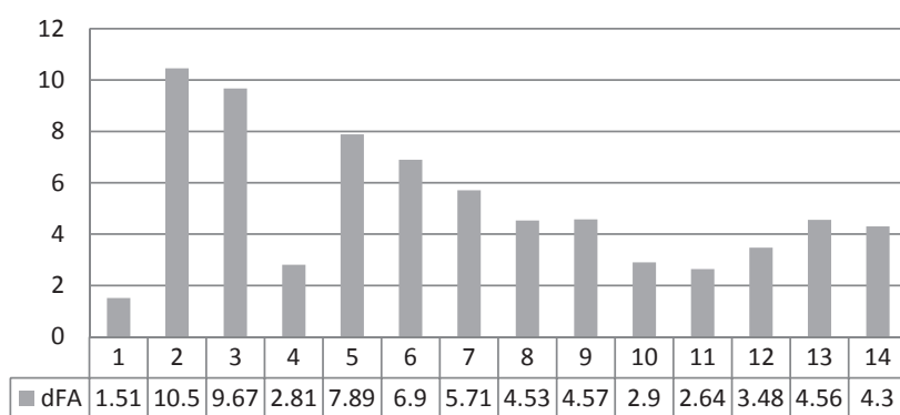
3: An increase in the fixed assets in million CZK of particular companies to increase the total production by 1% Source: own calculations
