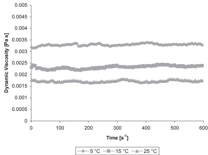
5: The dependence of viscosity of malt wort on the time
