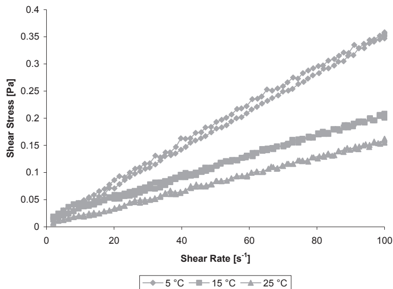
4: Hysteresis loops tests of hopped wort
