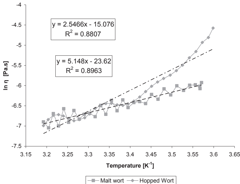
2: Evaluation of Arrhenius model of malt wort and hopped wort
