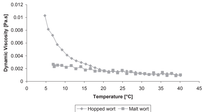
1: The dependence of dynamic viscosity on the temperature
