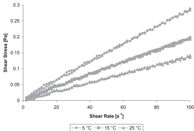
3: Hysteresis loops tests of malt wort
