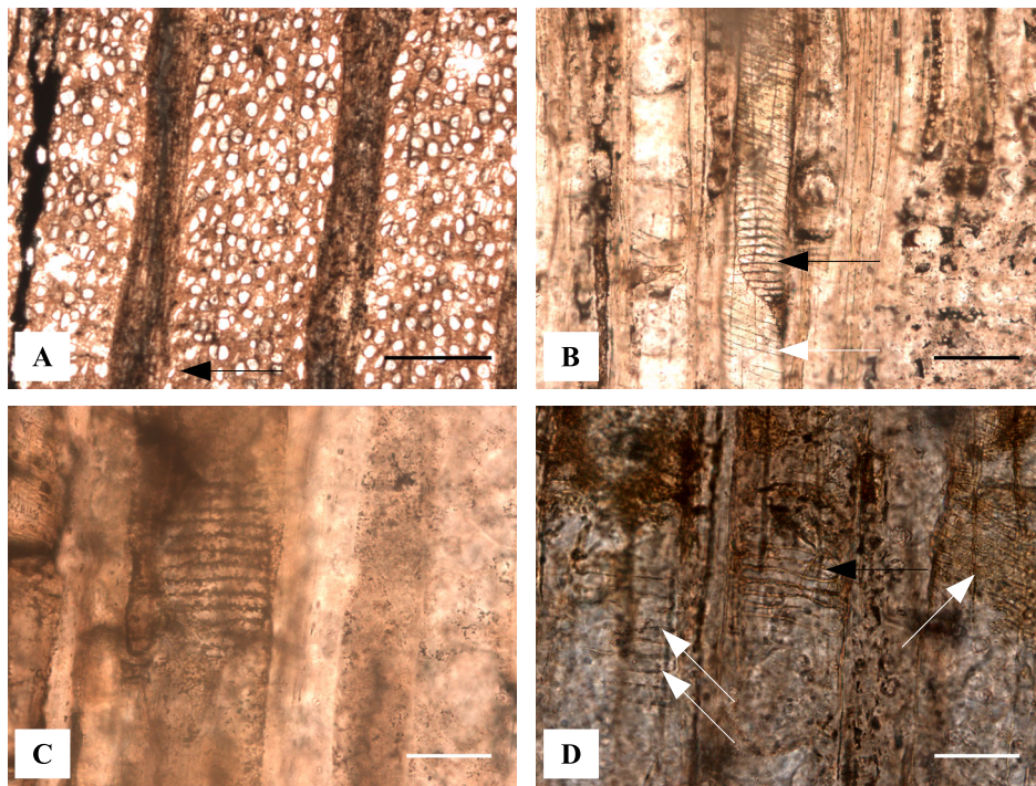
3: Microscopic observation of silicified wood: Spiroplatanoxylon mueller-stollii Süß (No. 10 – Gadas, MU) A – TS, section DR 0062, diffuse porous structure, vessels exclusively solitary, almost indistinct growth ring boundaries (see arrow), scale bar 500 µm. B – RLS, section DR 0063, vessels with scalariform perforation plates (black arrow) and helical thickenings (white arrow), scale bar 100 µm. C – RLS, section DR 0063, detail of vessel with scalariform perforation plates, scale bar 50 µm. D – RLS, section DR 0063, detail of helical thickenings (white arrows) and scalariform perforation plates (black arrow), scale bar 50 µm.
