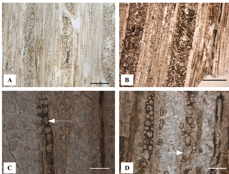
5: Microscopic observation of silicified wood: Spiroplatanoxylon mueller-stollii Süss (No. 10 – Gadas, MU) A – TLS, section DR 0064, multiseriate rays, scale bar 500 \mu\text{m} . B – TLS, section DR 0066, multiseriate rays, scale bar 500 \mu\text{m} . C – RLS, section DR 0063, axial parenchyma cells: detail of chambered crystalliferous cells (see arrow), scale bar 50 \mu\text{m} . D – RLS, section DR 0063, axial parenchyma cells: crystals in idioblasts (arrow), scale bar 50 \mu\text{m} .
