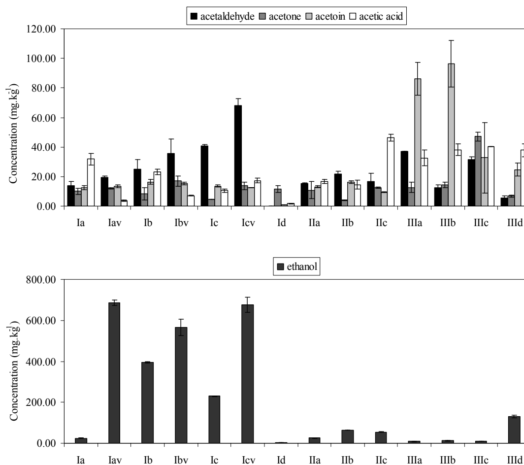
I: Comparison of chosen sensory active compounds in yogurt samples ( \text{mg}\cdot\text{kg}^{-1} )
